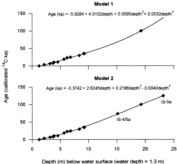
Fig. 2. Age-vs.-depth relations at Carp Lake based on Models 1 and 2 (see text for discussion). Dates are listed in Table 1.
