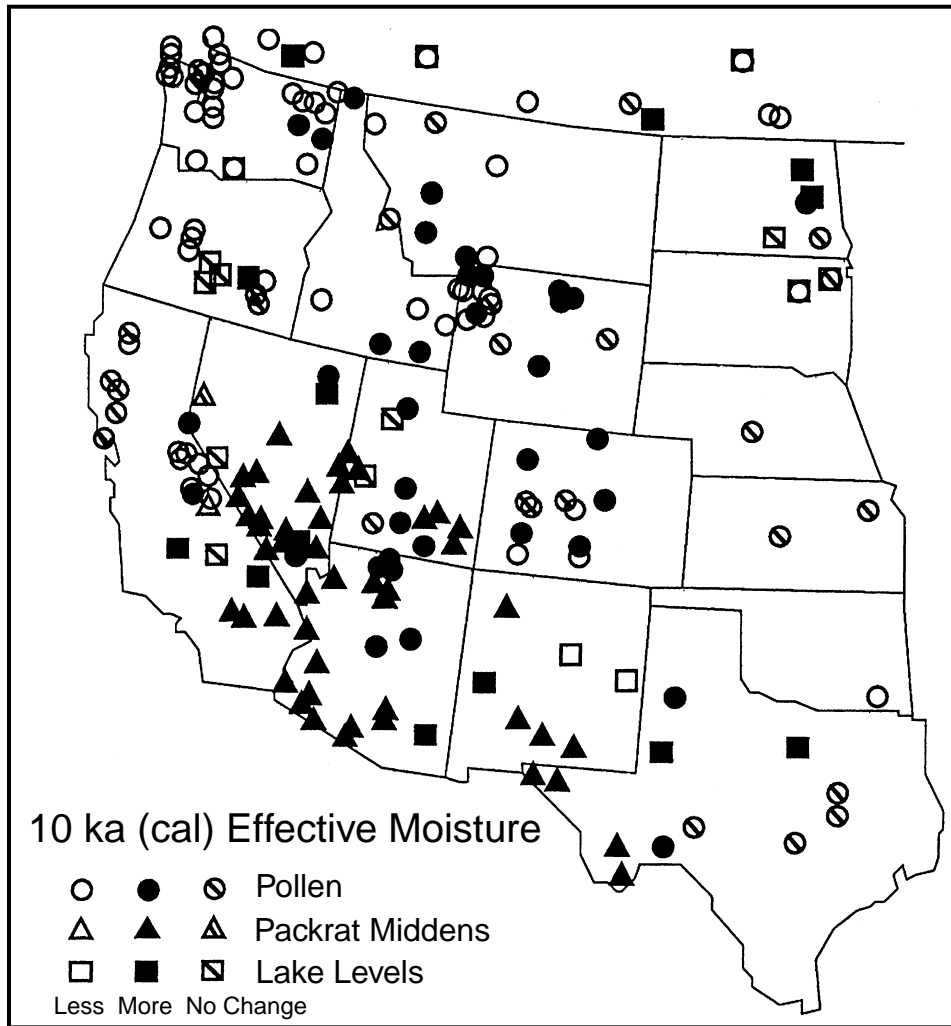
FIGURE 16: Effective moisture map for 10 ka for the western United States (Mock and Brunelle-Daines 1999).
