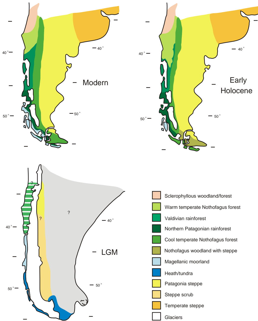
FIGURE 13: Comparison of modern, early Holocene, and full glacial vegetation in Patagonia, based on inferences from fossil pollen data.
