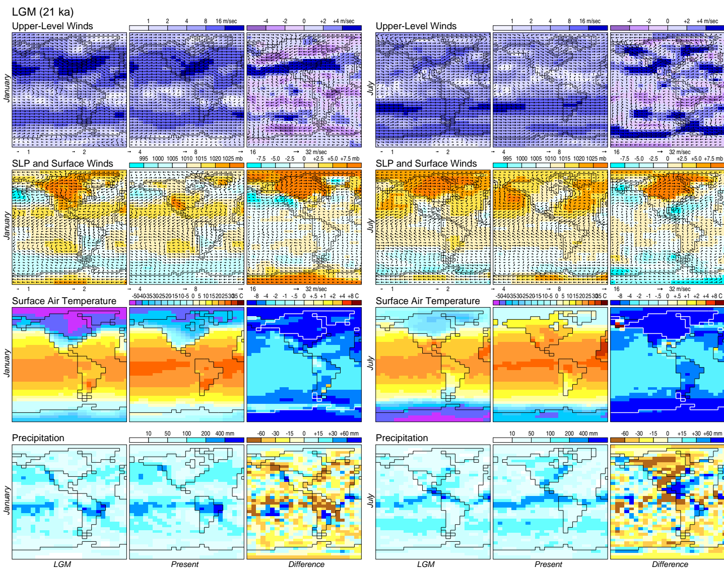
FIGURE 10: Simulated upper-level wind speed and direction, sea level pressure (SLP) and surface winds, surface air temperature, and precipitation for the last glacial maximum (LGM) for January and July.
