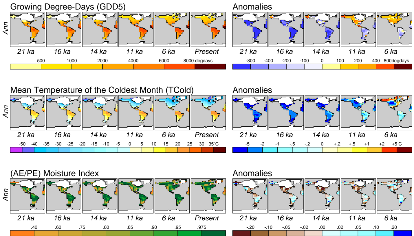
FIGURE 9: Temporal variations in bioclimatic variables: (top) growing degree-days ( 5^{\circ}\text{C} base), (middle) mean temperature of the coldest month, and (bottom) effective moisture, expressed as the ratio of actual to potential evapotranspiration (AE/PE), and their anomalies.
