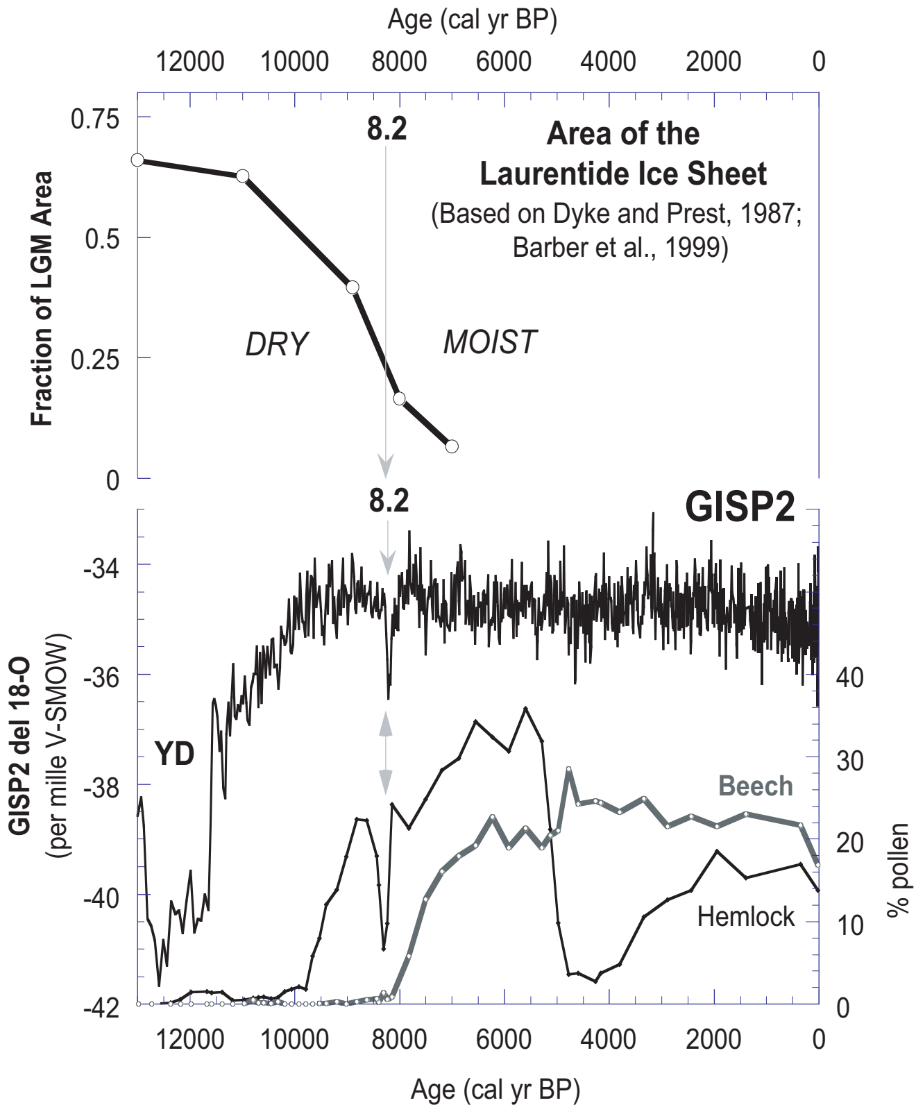
Pollen data from North Pond, MA (Whitehead and Crisman, 1978)
