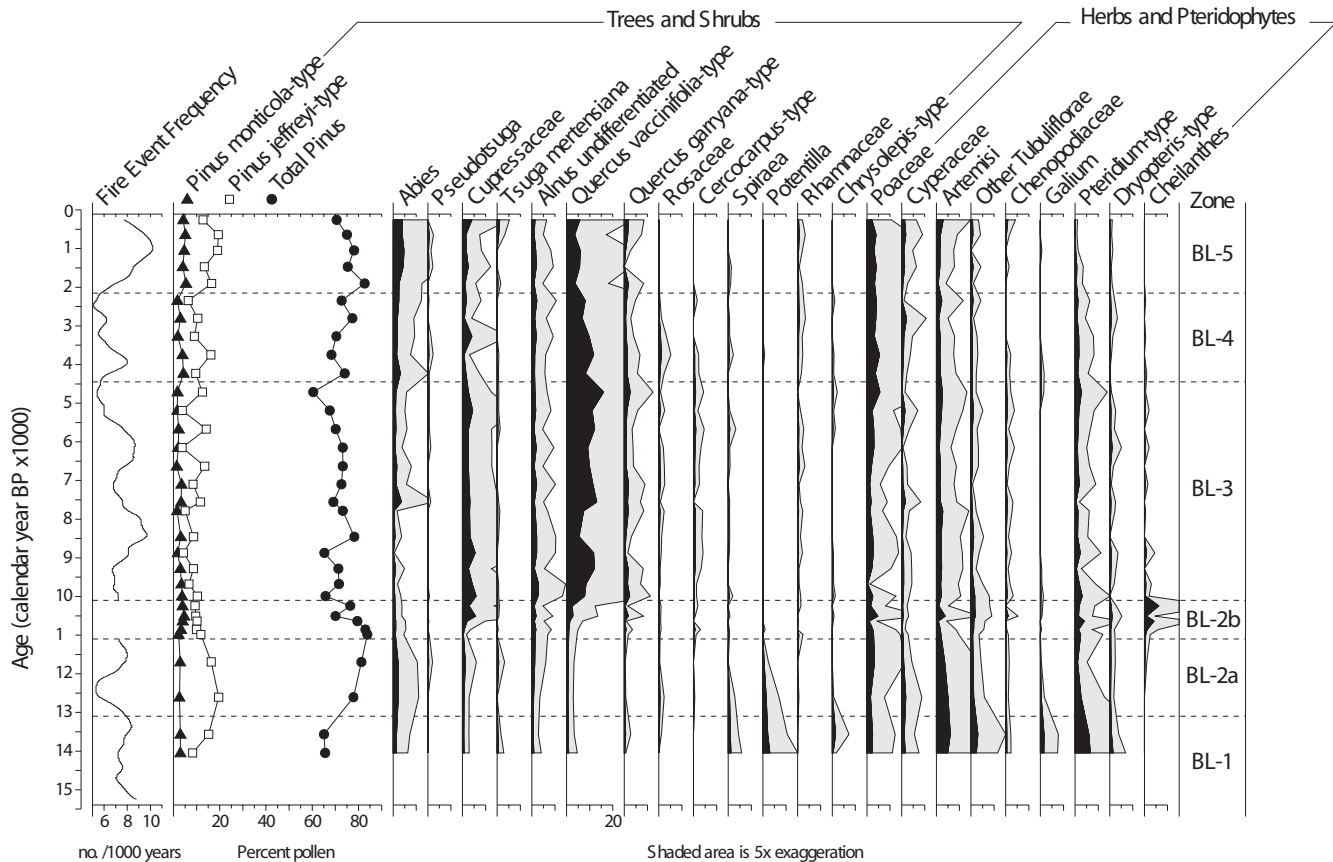
Figure 7 Fire-event frequency and pollen-percentage diagram of selected taxa for Bluff Lake. Shaded area represents exaggeration of 5x. Fire events span 24 to 180 years.
