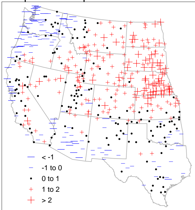
Temperature Departures
