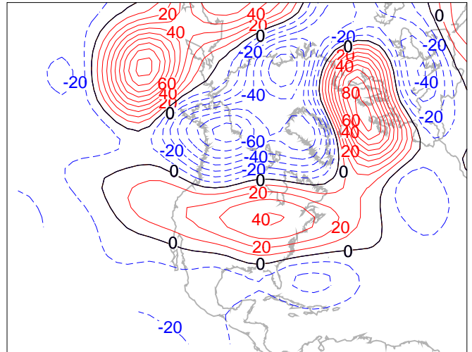
Precipitation Percentiles
