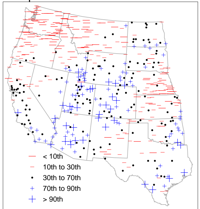
Precipitation Percentiles
