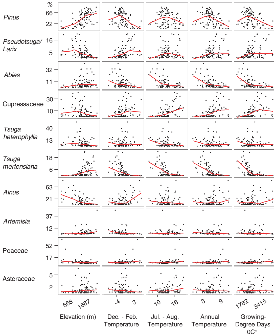
Figure 5. Scatter diagrams (MINITAB 1998) showing the abundance of selected pollen types plotted against environmental variables. Lowess curves show the locally weighted regression of the relationship of pollen to climatic variables. Lowess curves were created with a 3-step window and 0.7 degree of smoothing.
