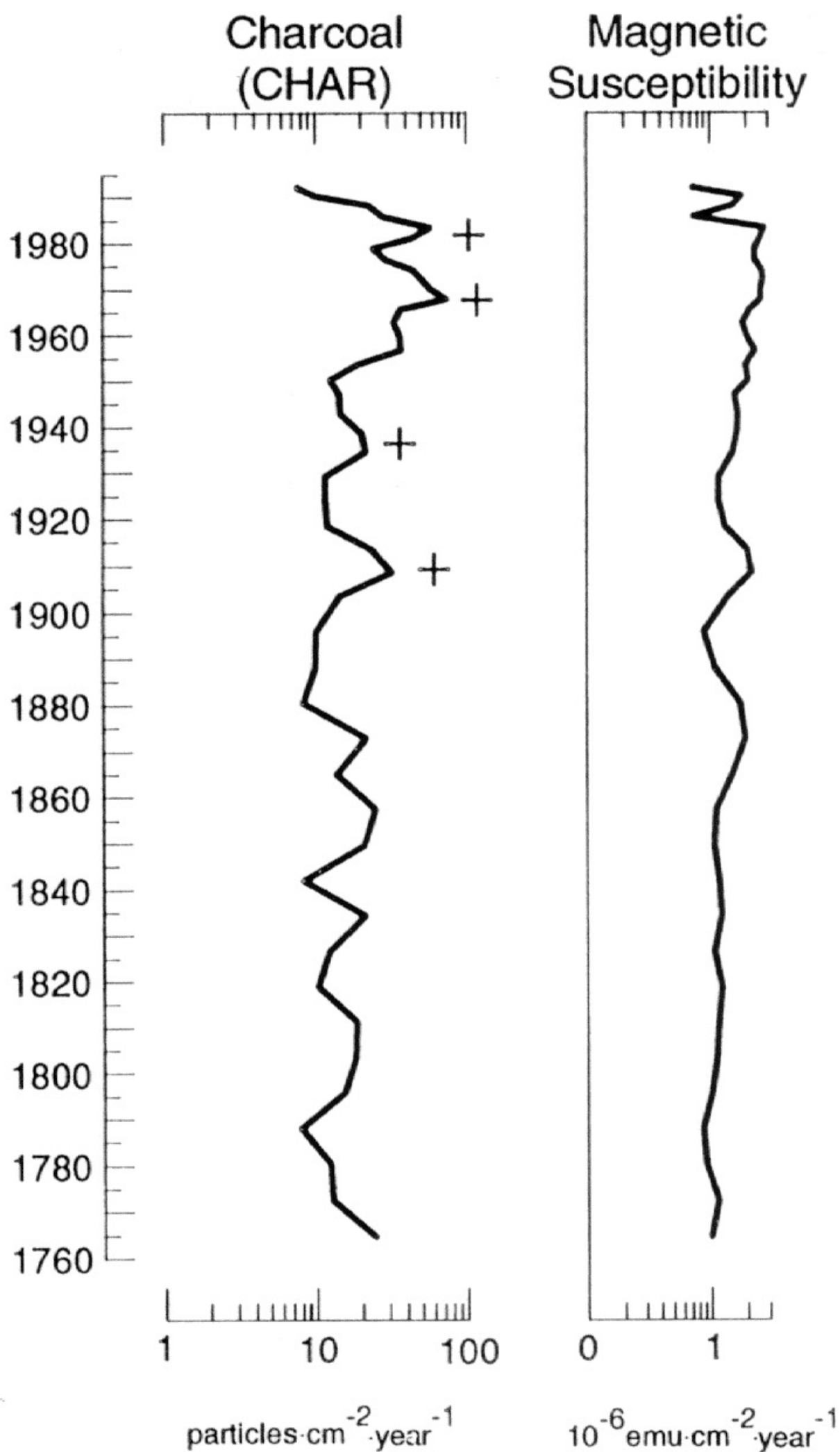
Fig. 3. Log-transformed charcoal (CHAR) and magnetic susceptibility accumulation rates plotted against age in the short core. Core intervals with a plus sign are associated with known or suspected watershed fires in 1982, 1967, 1934, and 1910.
