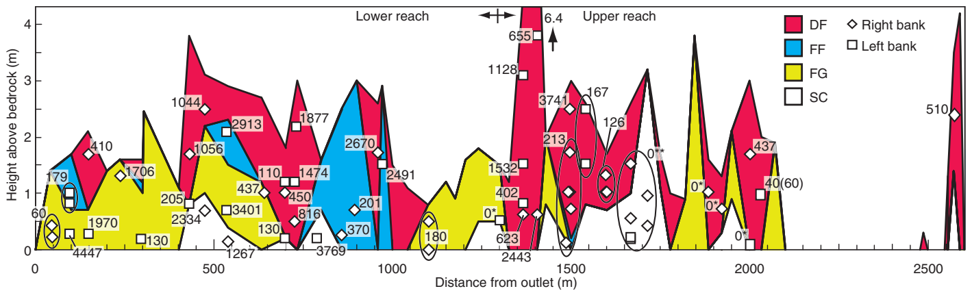
Figure 2. Cut-bank height at surveyed cross sections versus distance from outlet. Colors indicate deposit type: DF—debris flows; FF—fluvial fine; FG—fluvial gravels; SC— sediment covering bedrock (depth inferred). Interpolation between points is for illustrative purposes only; stratigraphic units are too numerous and localized to show legibly. Deposit ^{14}\text{C} ages (and 1\sigma errors where \geq 50 ^{14}\text{C} yr) are shown as right bank (diamonds) and left bank (squares). In all cases, actual samples for ^{14}\text{C} dating were found within 2 m streamwise, 0.1 m vertical, and 0.5 m (excavated) lateral distance, respectively, of target locations, and were classified as detrital wood, detrital charcoal, wood, branch wood, streamlined branch wood (knots left by erosion of surrounding, softer wood), or wood bark. For detrital wood and charcoal, some samples comprised two or more small pieces. Encircled sampling points indicate where ages of higher samples were inferred from lower samples. Points with 0^* have post-A.D. 1950 ^{14}\text{C} ages; points with 0^{**} were not actually sampled, but all are within deposit inferred to date to A.D. 1996. All other points within SC were accessed by excavating bank-adjacent bed material. Failure of the law of superposition at (1) 727 m from the outlet may reflect old-wood deposition (Gavin, 2001); (2) 1365 m from the outlet is due to a bank collapse; and (3) 1496 m from the outlet is likely due to debris-flow entrainment and redeposition of older upstream fluvial deposits. For precise sample locations, characteristics, and age estimates, see the GSA Data Repository (see footnote 1).
