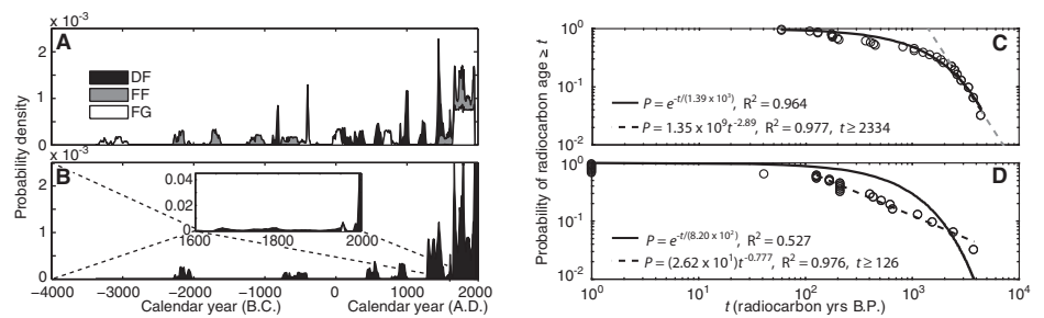
Figure 3. A, B: Normalized probability densities versus time (calibrated calendar dates from IntCal04 of Reimer et al. [2004a] and Bomb04NH1 of Hua and Barbetti [2004] for ^{14}\text{C} ages > 0 and F14C > 1 , respectively; cf. Reimer et al. [2004b]) for samples from lower (A) and upper (B) reaches of Bear Creek. Shading indicates different facies contributions: black is debris flow (DF); gray is fluvial fine (FF); and white is fluvial gravels (FG). Inset in B shows detail of post-A.D. 1600 probability densities with expanded time axis and compressed probability axis. C, D: Exceedance probability ( P ) versus ^{14}\text{C} age ( t , ^{14}\text{C} yr B.P.) for samples from lower (C) and upper (D) reaches of Bear Creek. Open circles are sample ages. Solid black lines are exponential distributions fit to all of the data, and dashed lines are power laws fit to the greater-age “tails” (equations shown with R^2 , fraction of variance explained). In C, gray dashed lines show extrapolations beyond the data used in the power-law fit.
