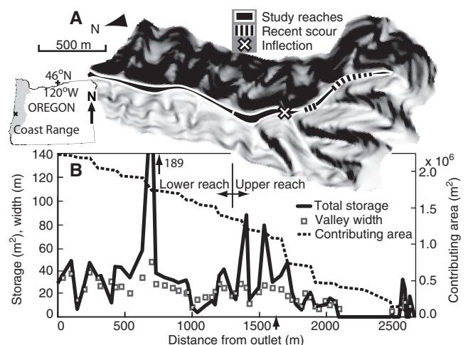
Figure 1. A: 10 m shaded relief map of Bear Creek basin, Oregon Coast Range, showing upper and lower study reaches (outlined in white). Hachures show locations of recent debris-flow scour. X (and arrow on distance axis in B) shows location of debris-flow–fluvial transition from power-law fitting method of Stock and Dietrich (2003); results of other methods were ambiguous. B: Cross-sectional areas of sediment stored above bedrock valley floor; valley width (distance between valley walls on deposit surface)
